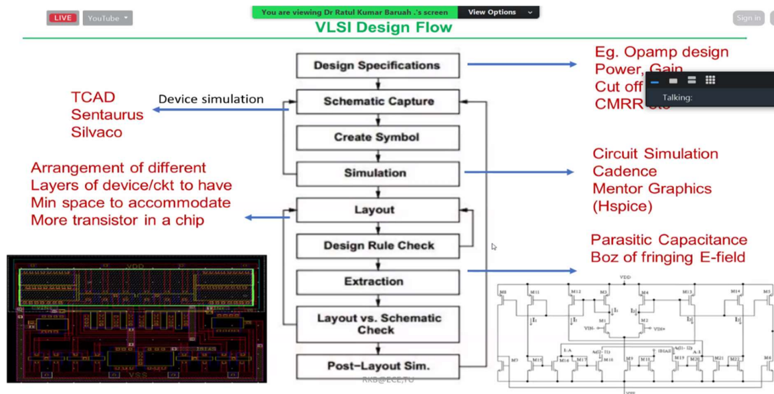
Typical VLSI Design Flow
